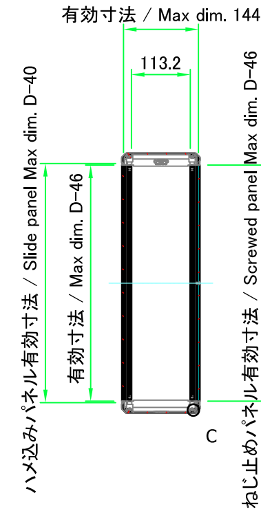
B-B (1:10)
